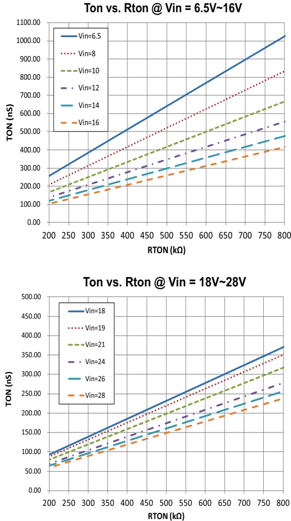
Figure 3. Ton vs. Rton Curves for AOZ2253EQI-30
