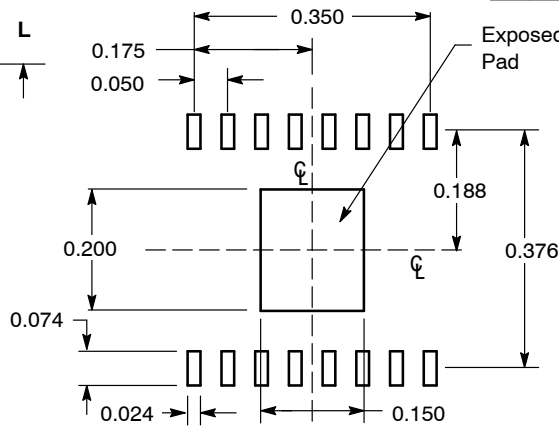
DIMENSIONS: INCHES
