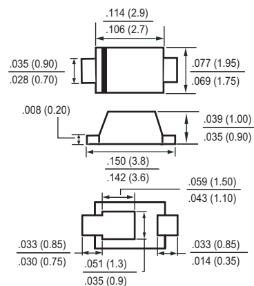
SOD-123FL
