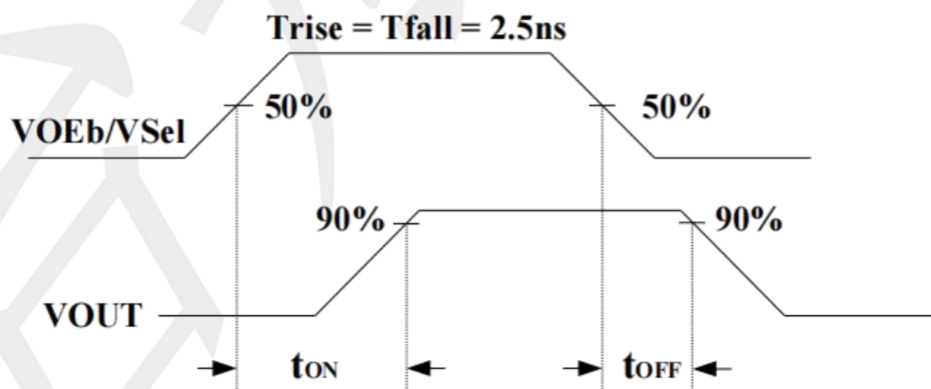
Test Circuit for Switch Times
