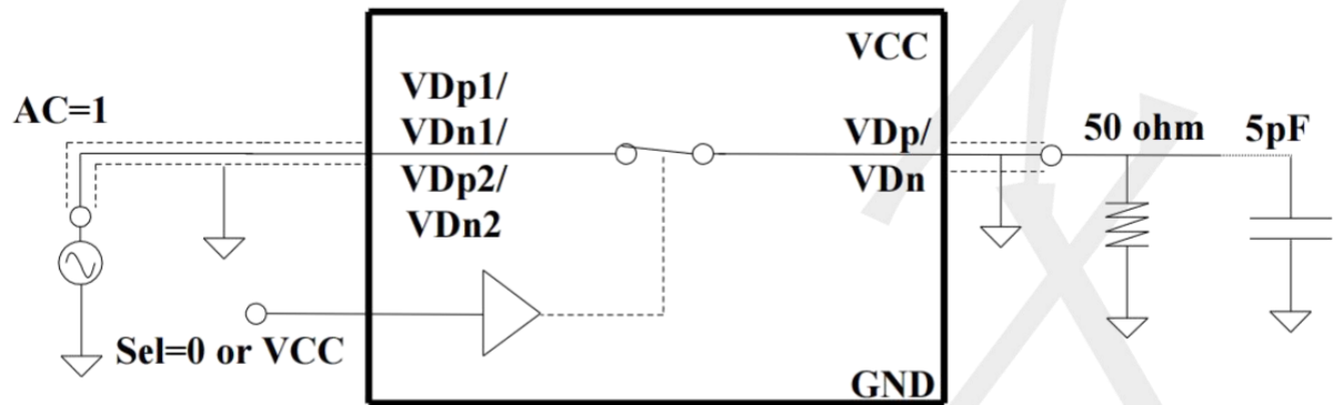
Test Circuit for Bandwidth
