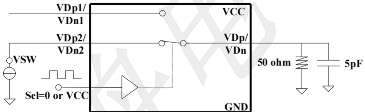
Test Circuit for Bandwidth
