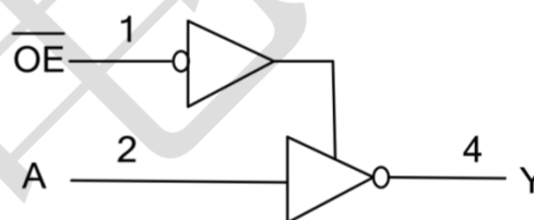
Logic symbol
