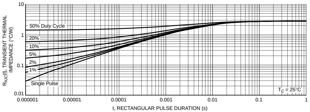
Figure 13. Thermal Response
