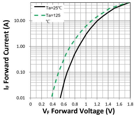
Figure 1. Forward Characteristic(typ.)
