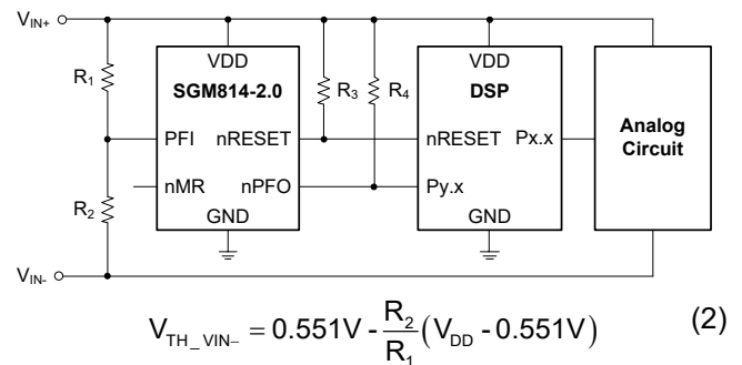
Figure 10. SGM814 Monitoring a Negative Voltage
