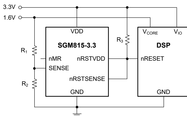
Figure 1. Typical Application Circuit Example
