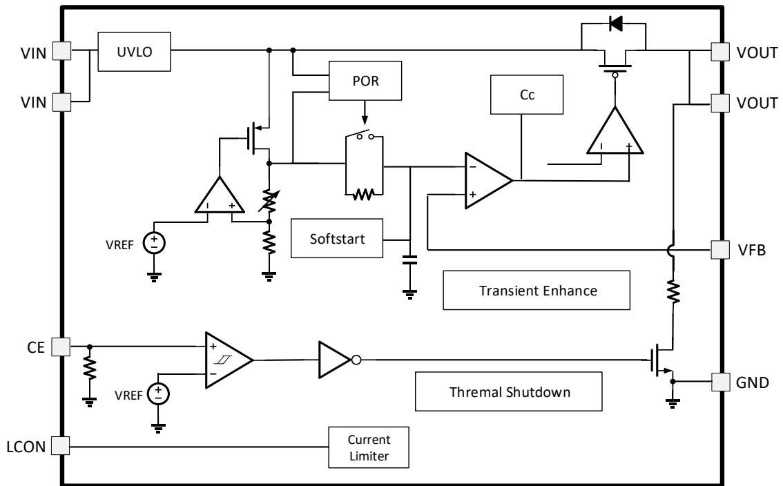
DFN1216-8 (8 PIN)
