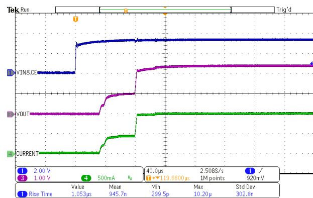
SUL6001D8-25
