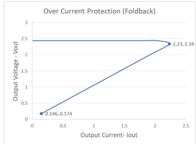
SUL6001D8-43
