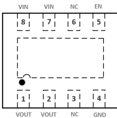
DFN 3030-8 Fixed
