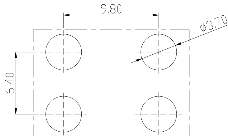
PCB LAYOUT
