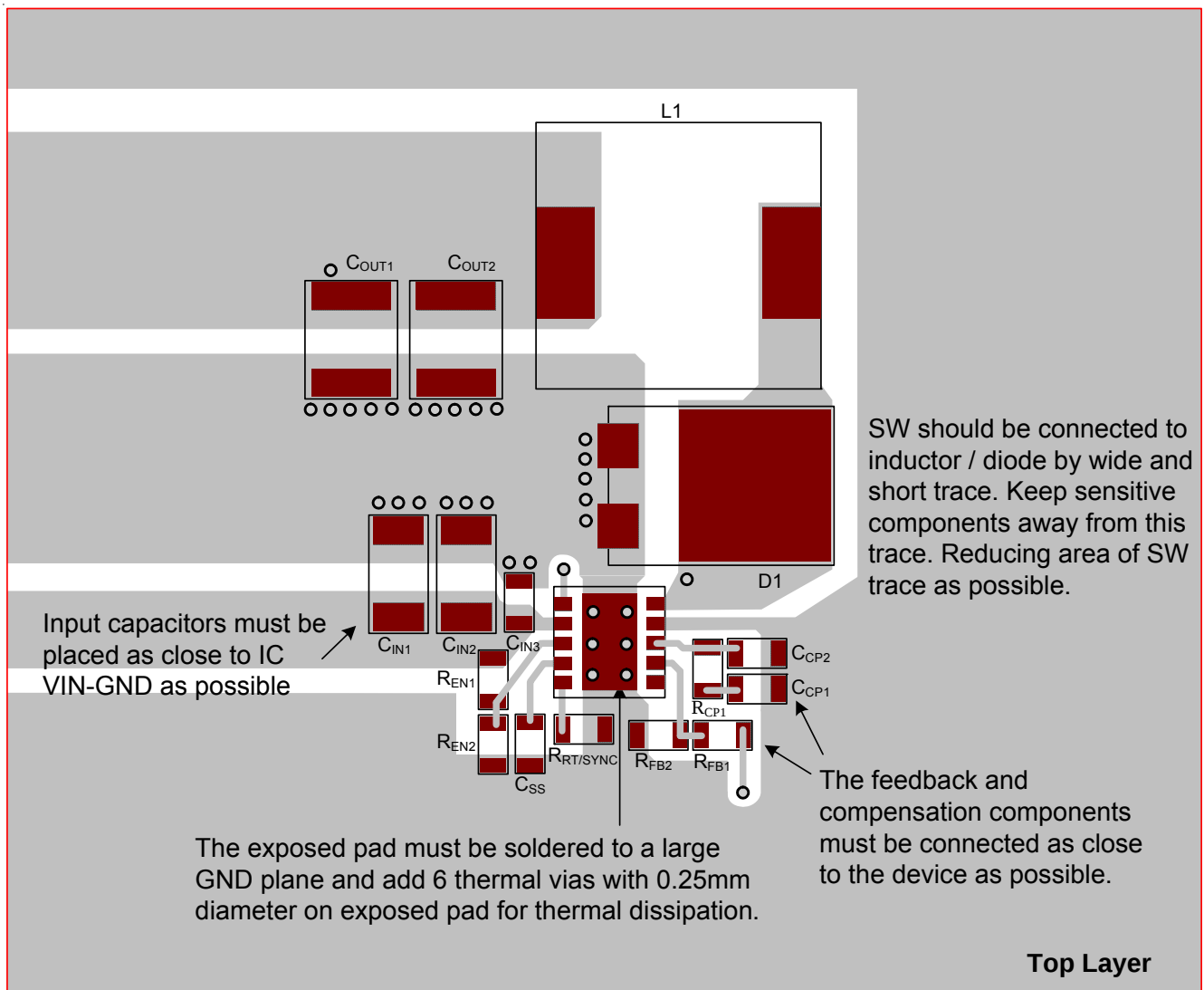
Figure 16. Layout Guide for RTQ6362GQW (Top Layer)
