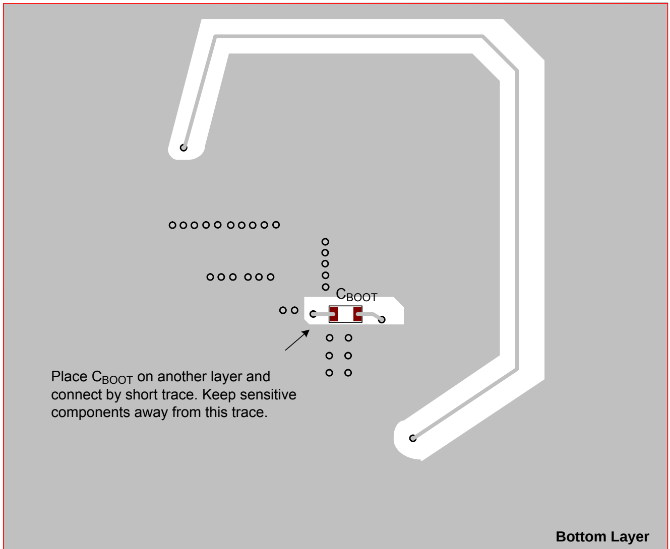
Figure 17. Layout Guide for RTQ6362GQW (Bottom Layer)
