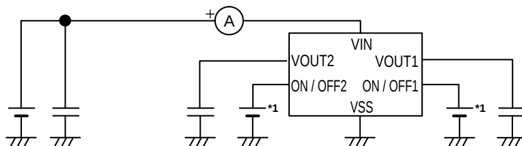
Figure 12 Test Circuit 2
