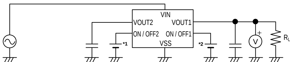
Figure 17 Test Circuit 7
