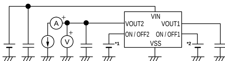
Figure 11 Test Circuit 1
