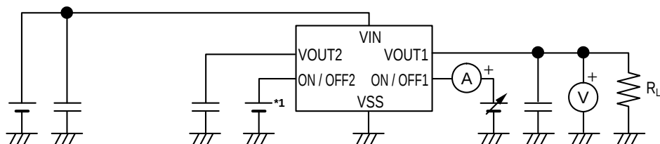
Figure 15 Test Circuit 5
