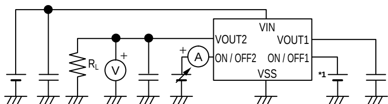
Figure 16 Test Circuit 6
