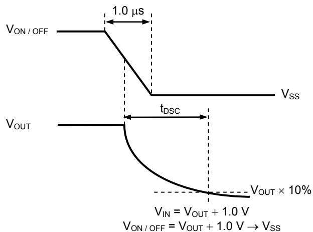
Figure 38 Test Condition of Discharge Time
