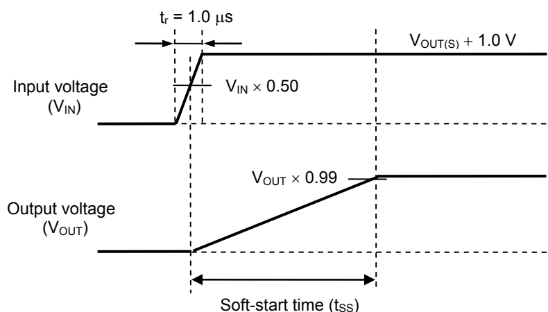
Figure 31 Basic Operation
