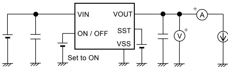
Figure 19 Test Circuit 6
