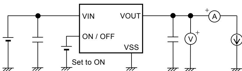
Figure 14 Test Circuit 1
