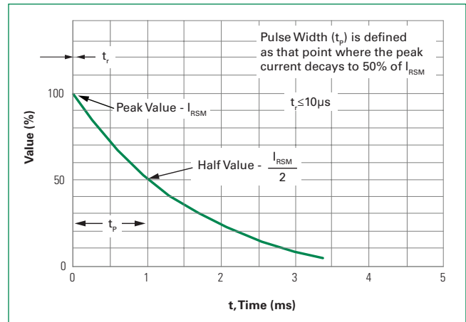
Figure 2. 10/1000 \mu s Pulse Waveform
