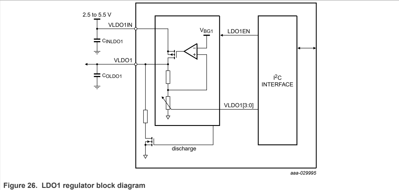
Figure 26. LDO1 regulator block diagram
