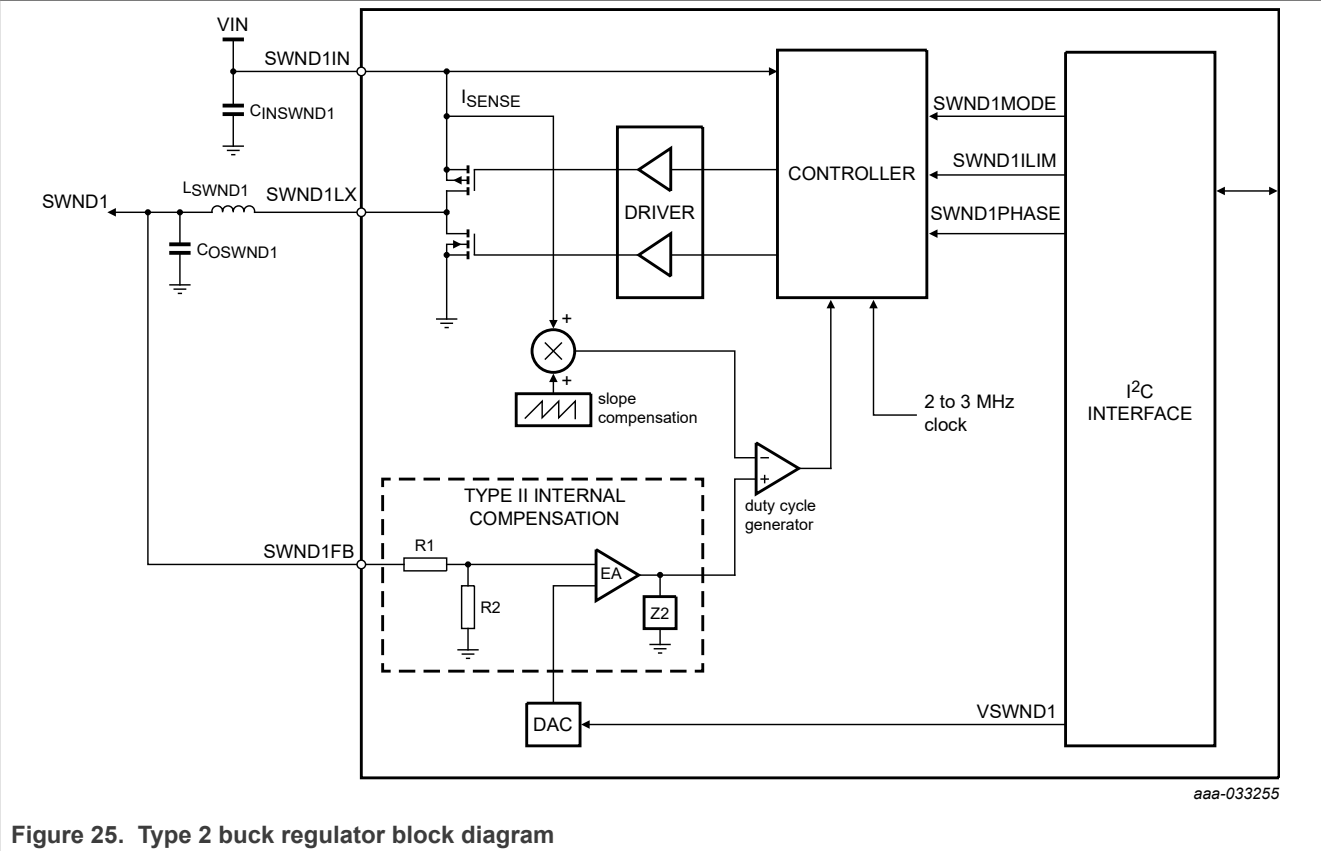
Figure 25. Type 2 buck regulator block diagram
