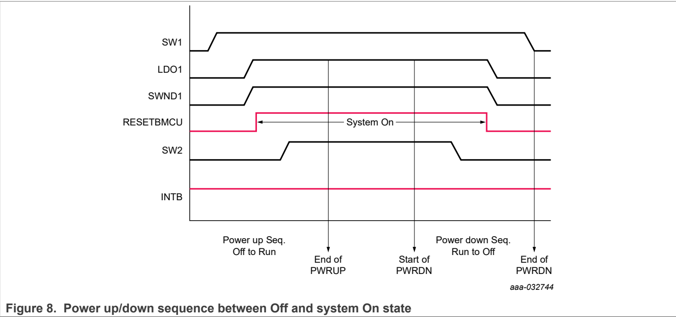
Figure 8. Power up/down sequence between Off and system On state When transitioning from Standby mode to Run mode, the power up sequencer is activated only if any of the external regulators is re-enabled during this transition. If none of the regulators toggle from Off to On and only voltage changes are being performed when entering or exiting Standby mode, the changes for the voltage regulators are made simultaneously rather than going through the power up sequencer. Figure 9 shows an example of the power up/down sequence when transitioning between Run and Standby modes.
