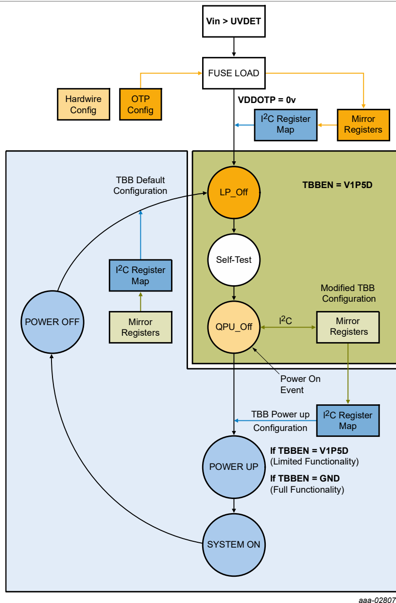
Figure 35. TBB operation diagram
