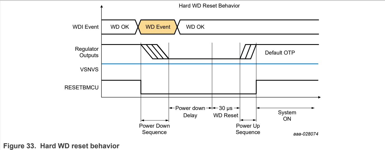
Figure 33. Hard WD reset behavior
