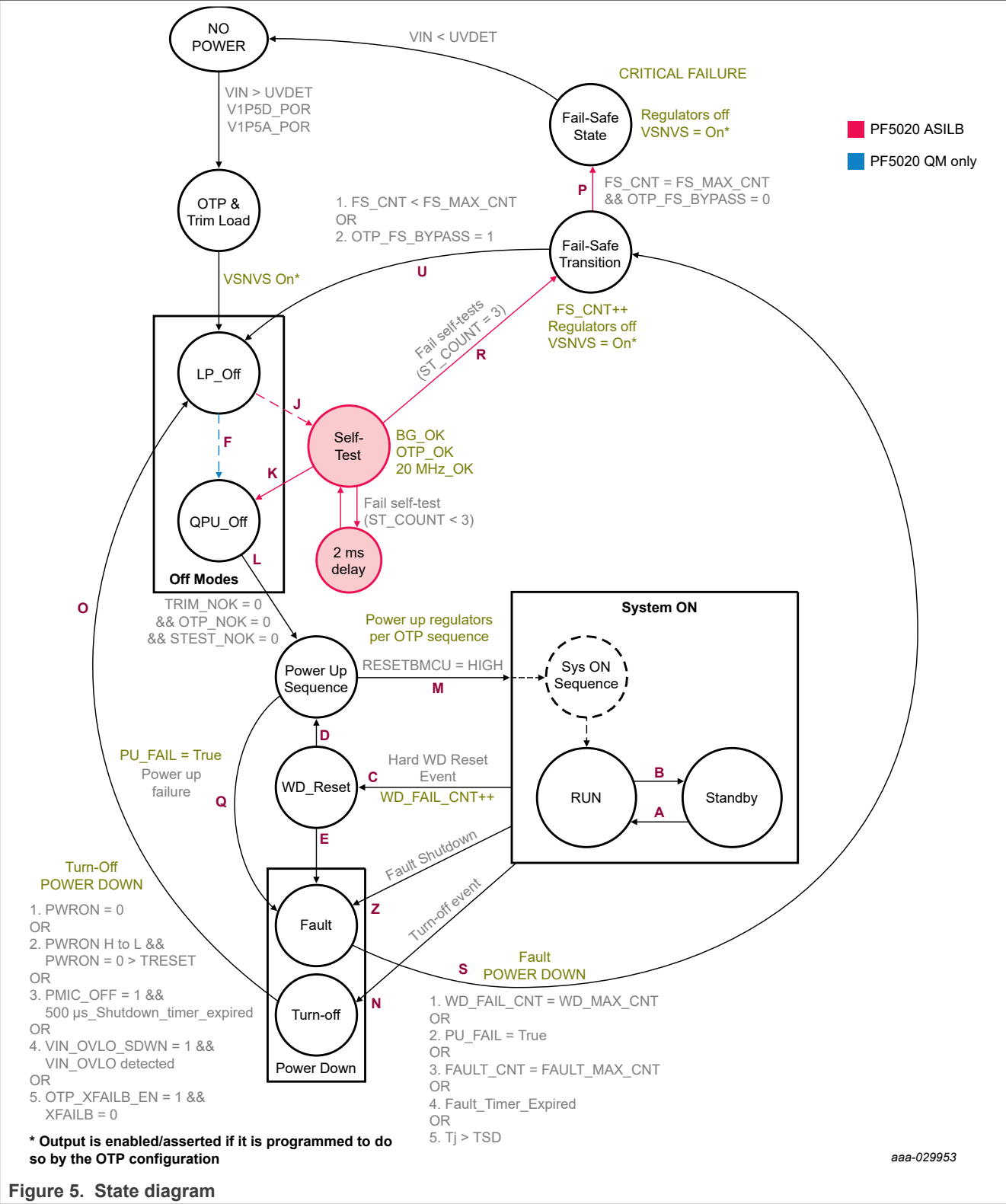
Figure 5. State diagram
