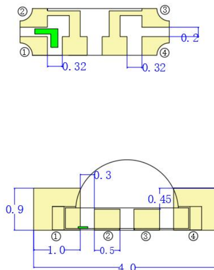
建议焊盘尺寸 Recommended Soldering Pattern
