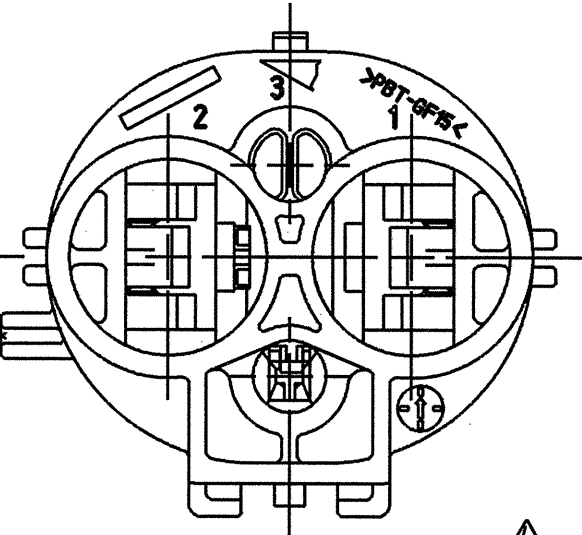
3P SEALED HYBRID CONNECTOR P.N. 7282-8496-30
