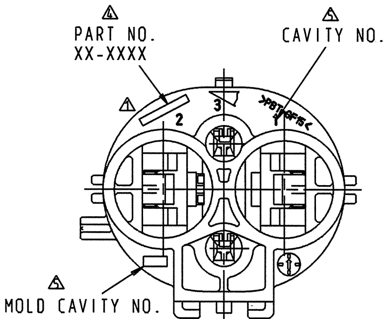
4P SEALED HYBRID CONNECTOR P.N. 7282-8497-90, 7282-8598-30
