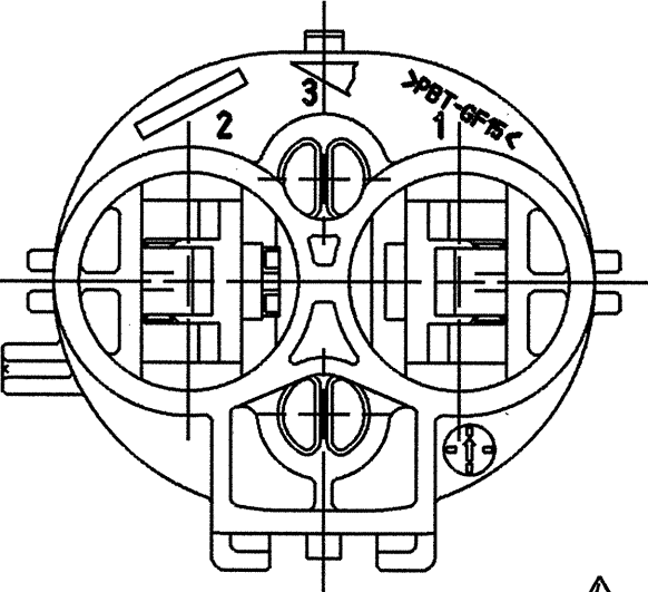
2P SEALED HYBRID CONNECTOR P.N. 7282-8495-10
