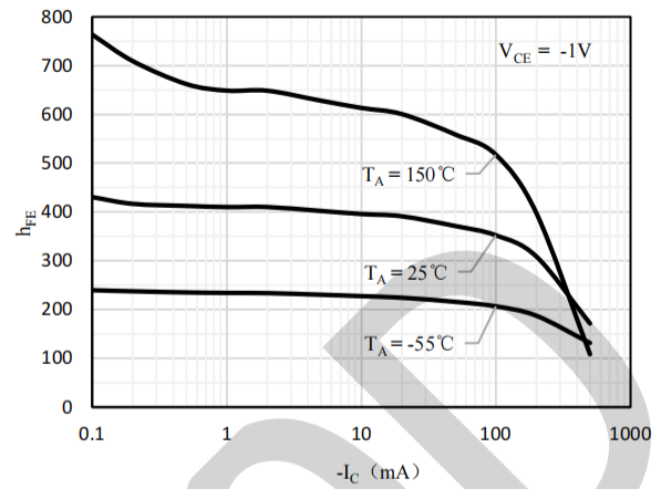
Fig 2 h_{FE} vs. I_C (BC807-25)
