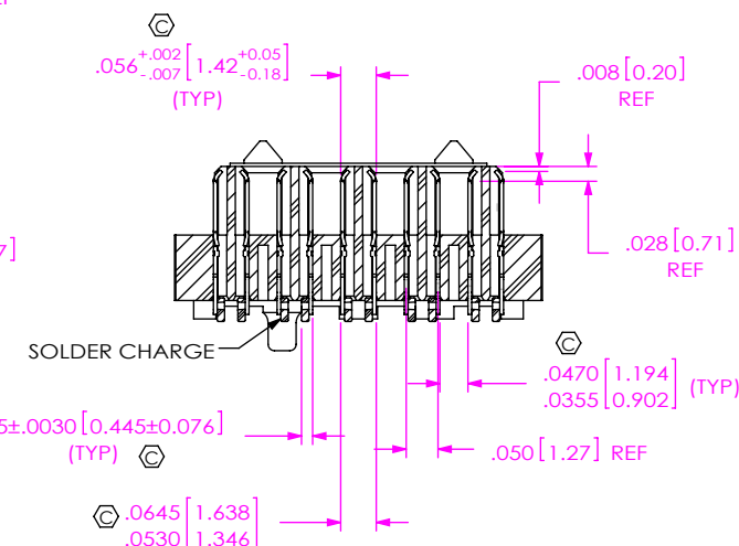
SECTION "C"-"C" SCALE 3 : 1
