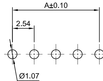
P.C.B LAYOUT TOLERANCE:±0.05
