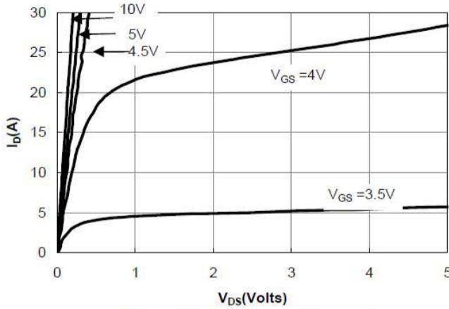
Figure 1: On-Regions Characteristics
