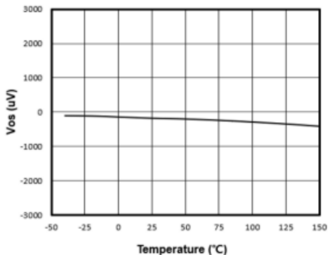
Figure 4. Offset Voltage vs. Temperature
