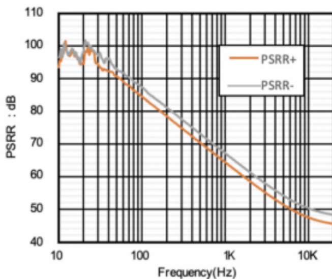
Figure 2. PSRR vs Frequency
