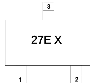
27E X= Device code Marking (Top View)
