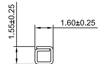
SEC:C-C
