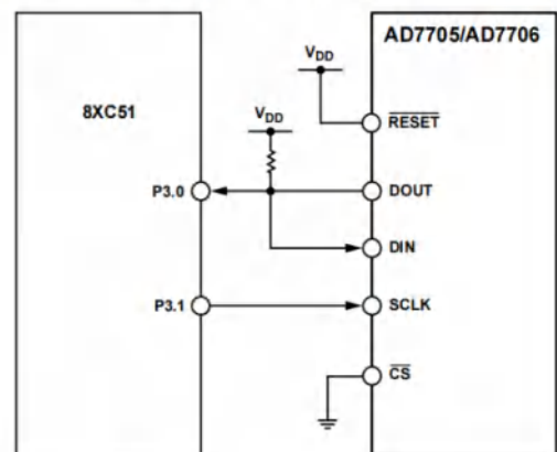
Figure 23. AD7705/AD7706-to-8XC51 Interface
