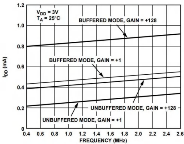
Figure 6. I_{DD} vs. MCLK IN Frequency @ 3 V
