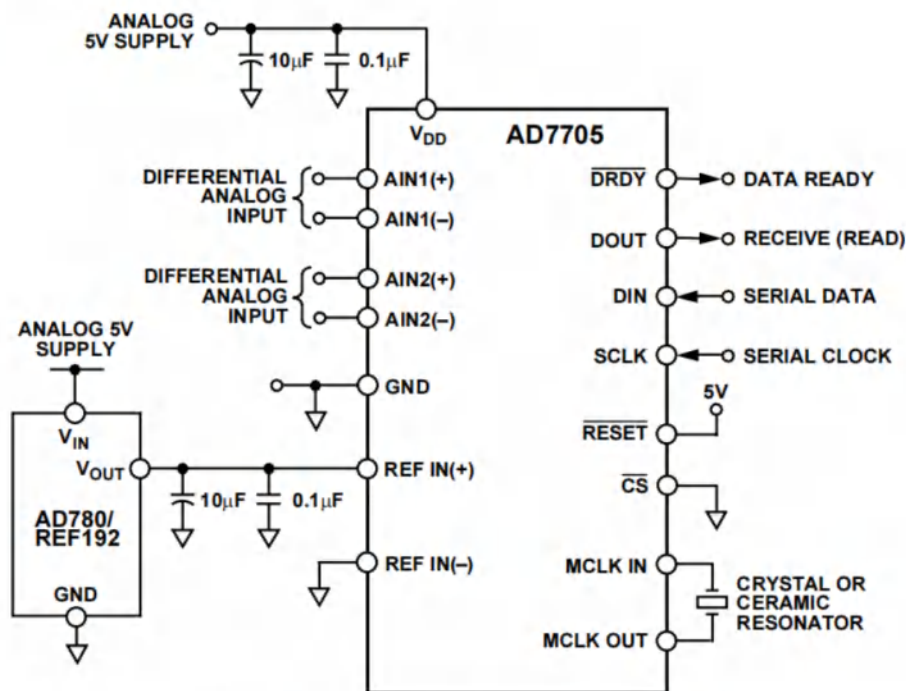
Figure 13. AD7705 Basic Connection Diagram
