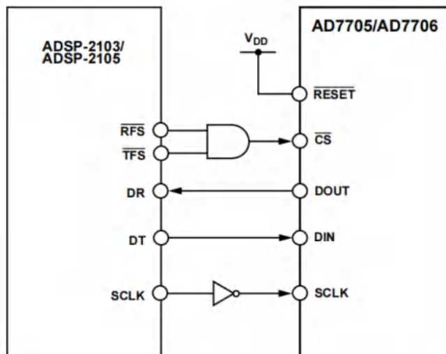
Figure 24. AD7705/AD7706-to-ADSP-2103/ADSP-2105 Interface
