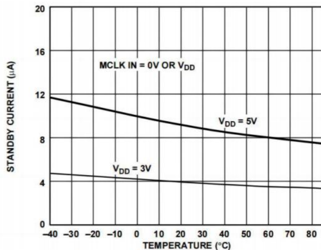
Figure 12. Standby Current vs. Temperature
