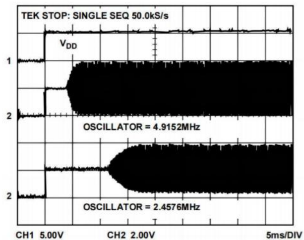
Figure 11. Crystal Oscillator Power-Up Time
