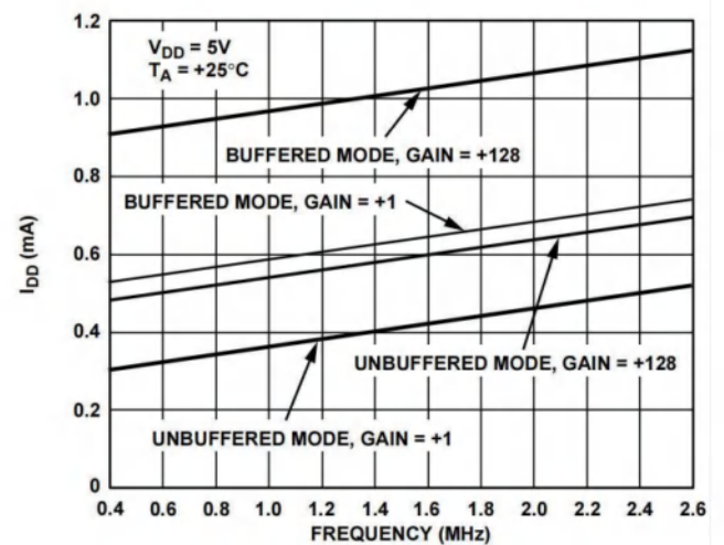
Figure 9. I_{DD} vs. MCLK IN Frequency @ 5 V
