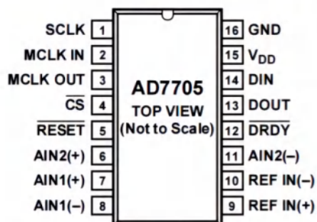
Figure 3. AD7705 Pin Configuration
