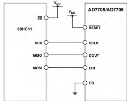
Figure 22. AD7705/AD7706-to-68HC11 Interface
