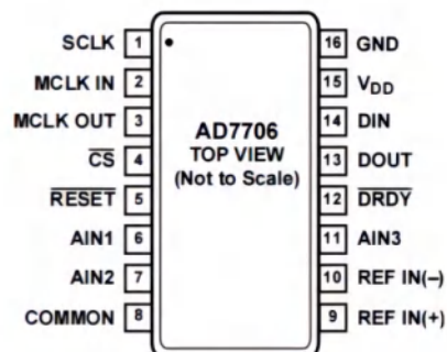
Figure 4. AD7706 Pin Configuration
