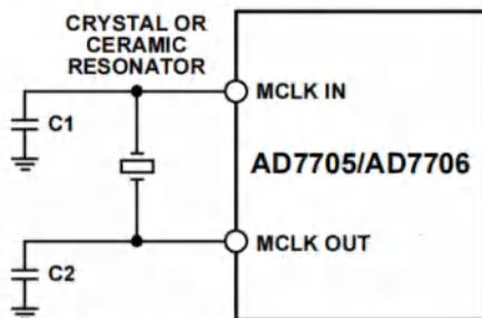
Figure 17. Crystal/Resonator Connection for the AD7705/AD7706
