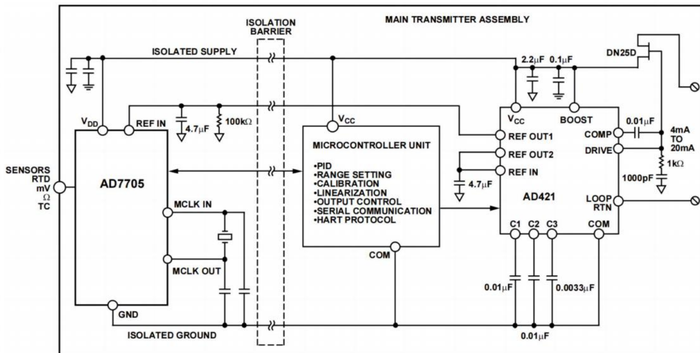
Figure 28. Smart Transmitter Using the AD7705
