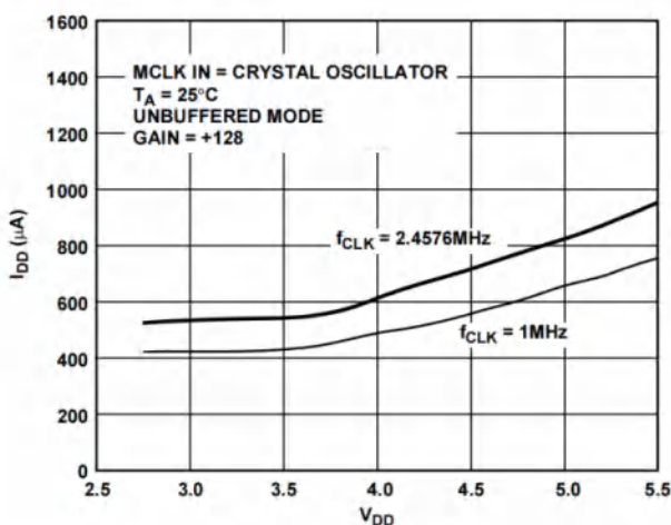
Figure 18. I_{DD} vs. Supply Voltage
