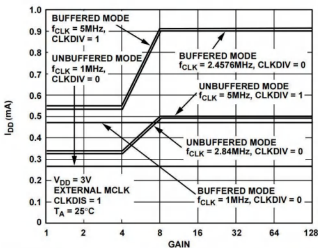
Figure 7. I_{DD} vs. Gain and Clock Frequency @ 3 V
