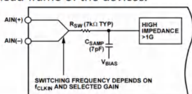
Figure 14. Unbuffered Analog Input Structure
