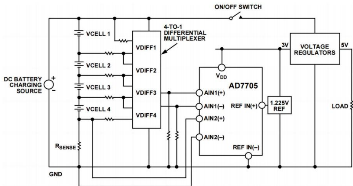
Figure 29. Battery Monitoring Using the AD7705
