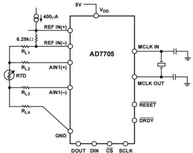
Figure 27. RTD Measurement Using the AD7705
