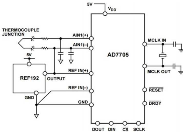
Figure 26. Temperature Measurement Using the AD7705
