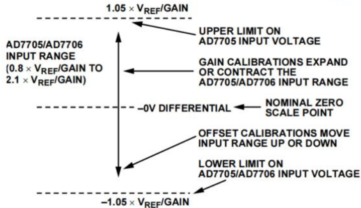
Figure 16. Span and Offset Limits
