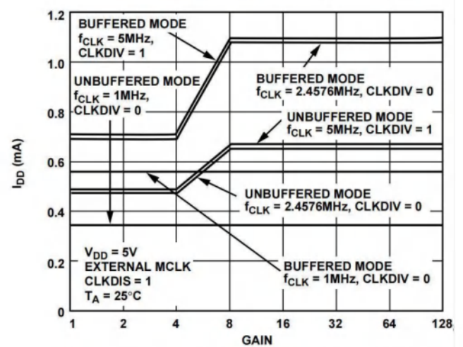
Figure 10. I_{DD} vs. Gain and Clock Frequency @ 5 V
