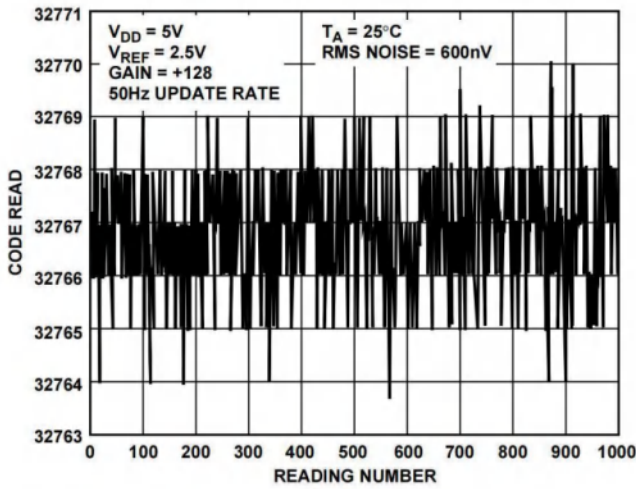
Figure 5. Noise @ Gain = +128 With 50 Hz Update Rate
