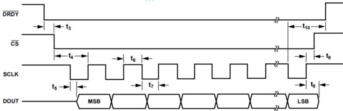
Figure 19. Read Cycle Timing Diagram
