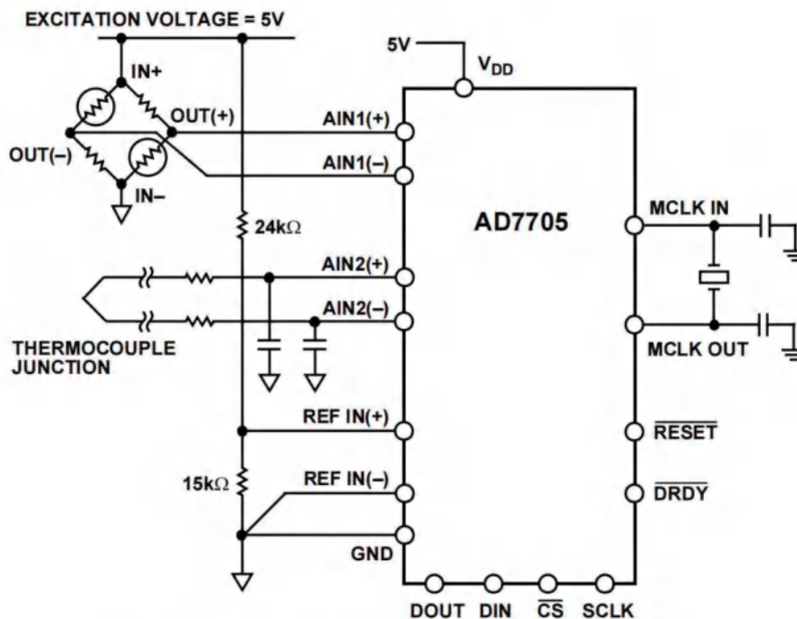
Figure 25. Pressure Measurement Using the AD7705
