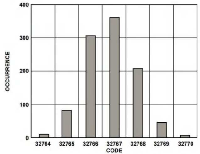
Figure 8. Histogram of Data in Figure 5
