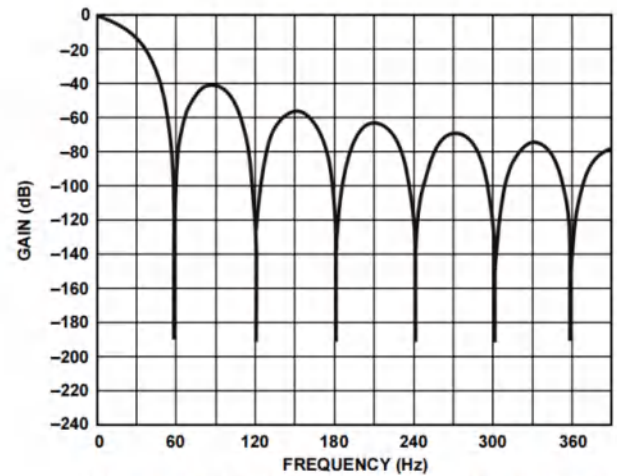
Figure 15. Frequency Response of AD7705 Filter
