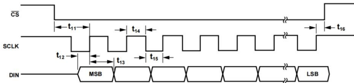
Figure 20. Write Cycle Timing Diagram
