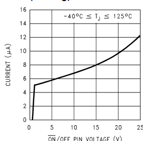
ON/OFF Pin Current (Sinking)
