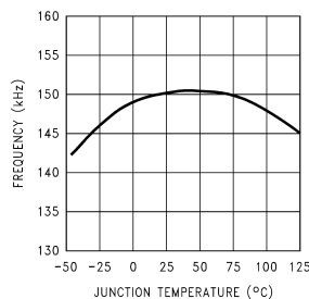
Switching Frequency
