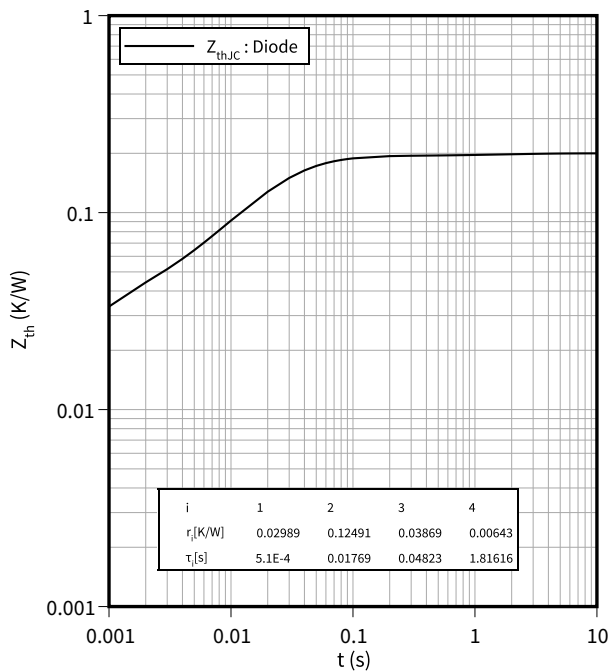
Transient thermal impedance , Diode, Inverter
