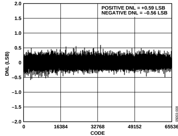
Figure 8. Differential Nonlinearity vs. Code
