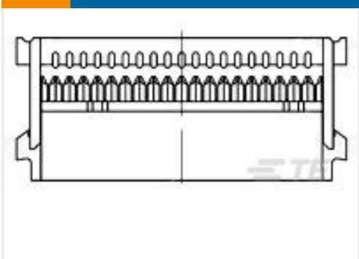
TE Part #1658526-5 609-1041LF FEM SOCKET,LEAD FREE
