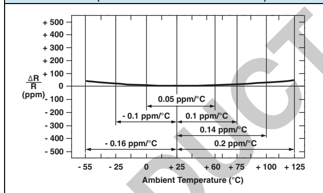
FIGURE 3 - TYPICAL TCR CURVE Z-FOIL
