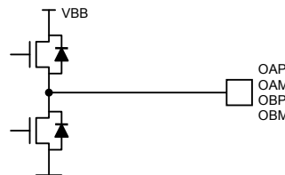
Figure 19i: Phase Outputs
