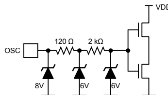
Figure 19f: OSC Input
