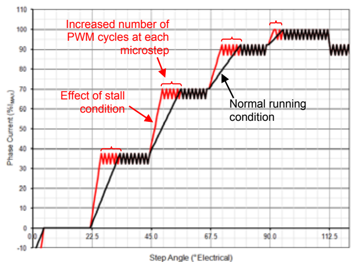
Figure 3. Effect of stall condition on current rise
