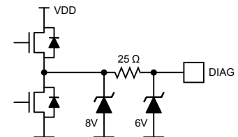
Figure 19j: DIAG Output
