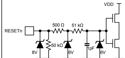
Figure 19g: RESETn Input
