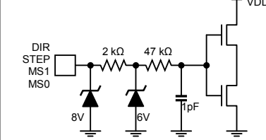
Figure 19c: DIR, STEP, MS1, MS0 Inputs
