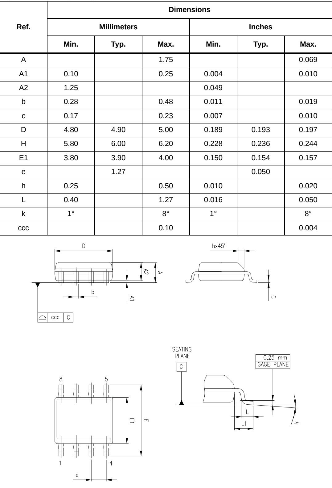
Figure 1. SO-8 package mechanical data
