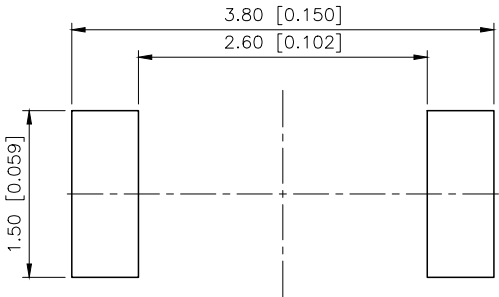
PCB SOLDER LAND DIMENSIONS
