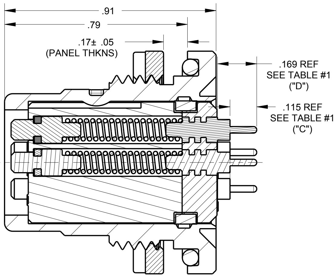
SECTION Z-Z SCALE 4.000
