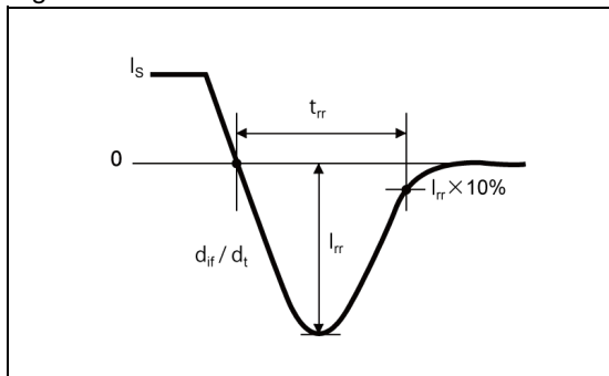
Fig.4-2 trr Waveform
