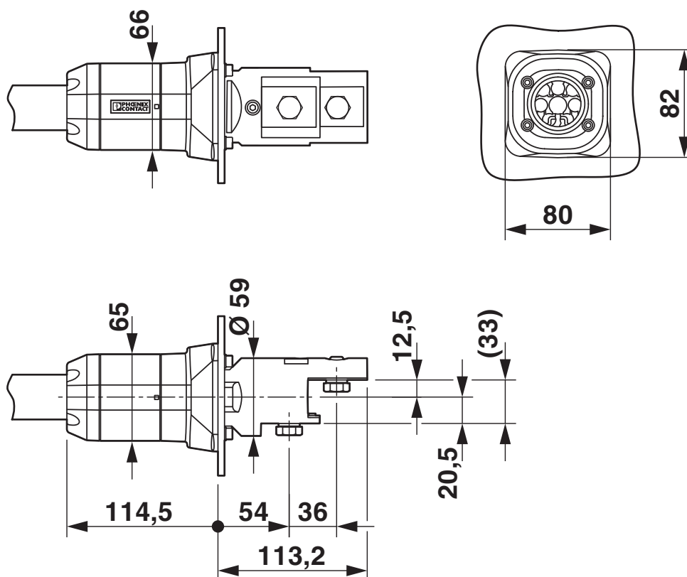
Straight panel feed-through
