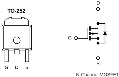
N-Channel MOSFET
