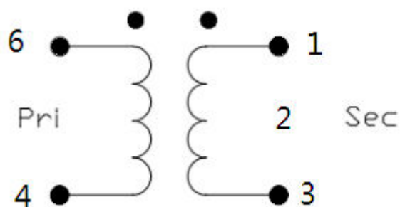
SCHEMATIC
