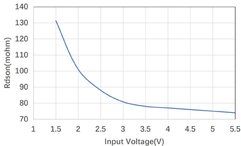
R_{ON} vs. V_{IN} ( V_{EN}=V_{IN} , I_{LOAD}=200\text{mA} )
