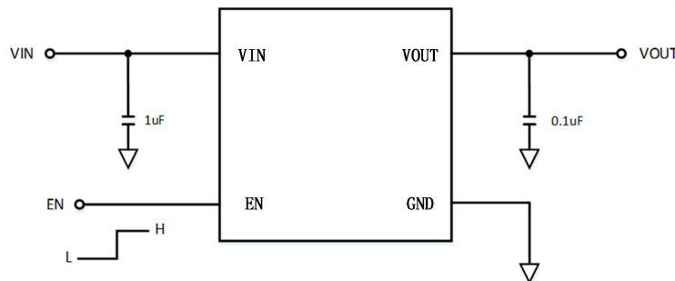
Fig. 3 Typical Applications
