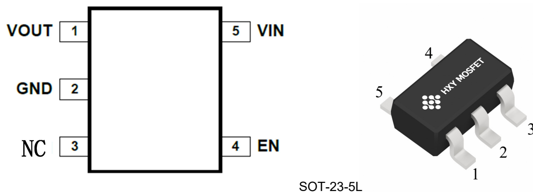
Fig. 1 Pin Information (Top View)
