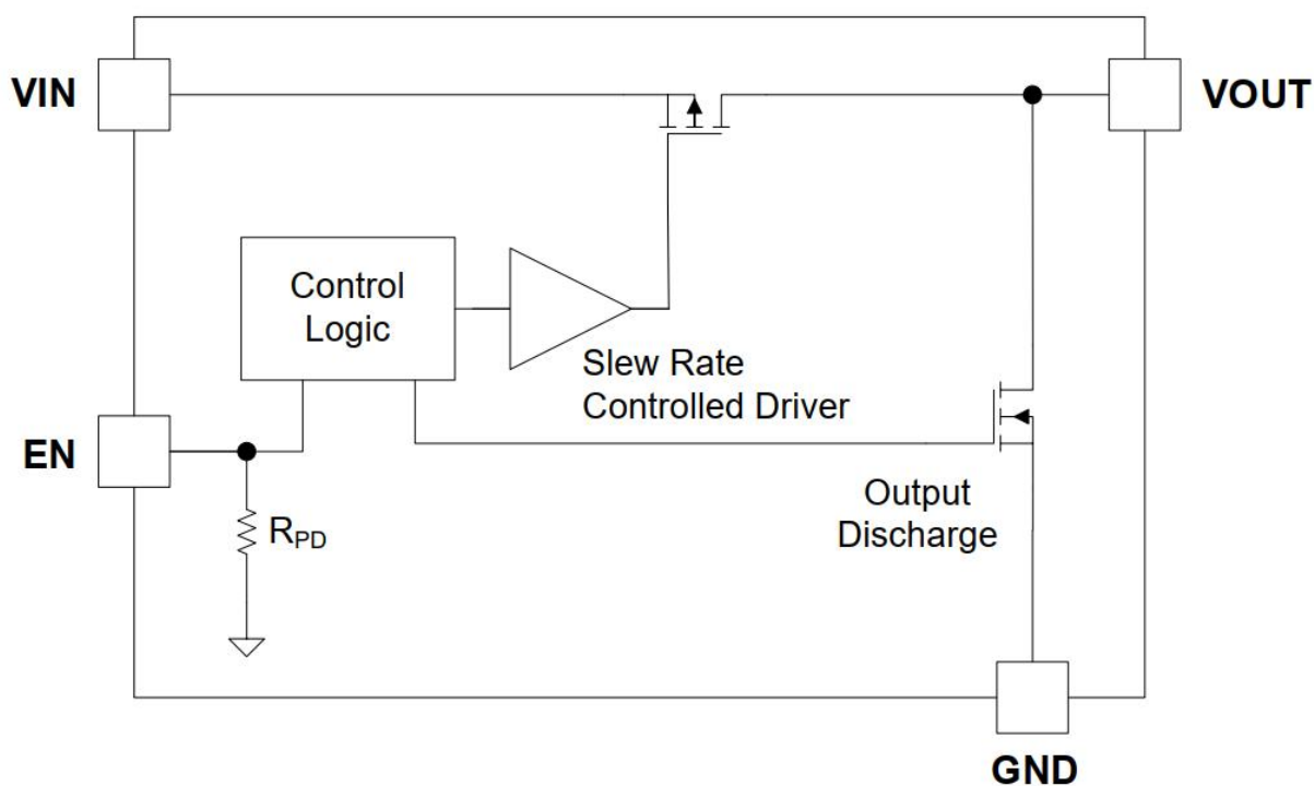
Fig. 2 Block Diagram
