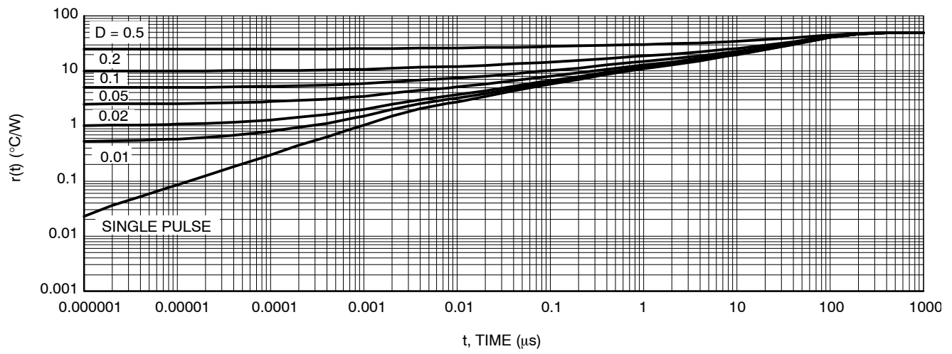
Figure 13. Thermal Response
