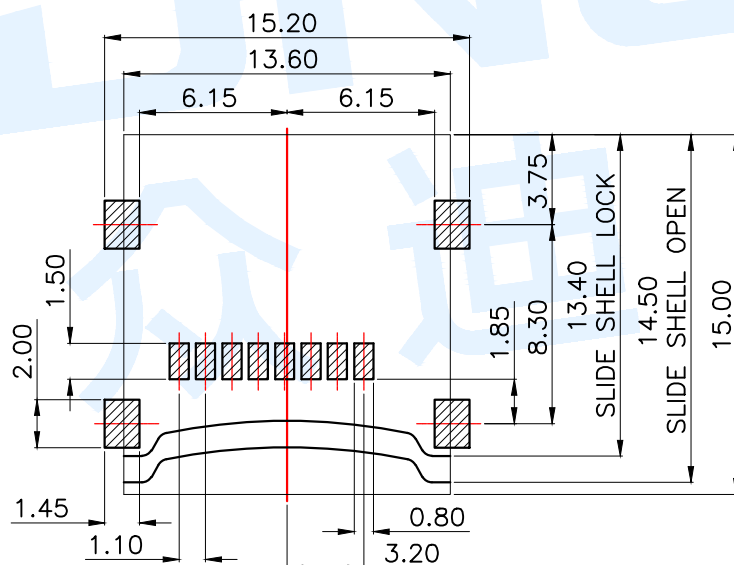
RECOMMENDED P.C.B HOLE LAYOUT COMPONENT SIDE VIEW(TOLERANCE: +/-0.05)
