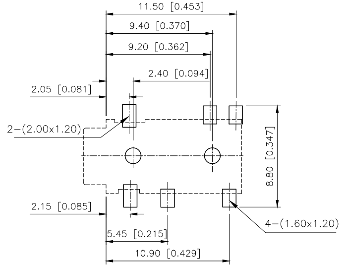
PCB LAYOUT
