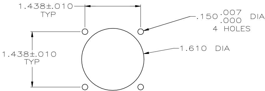
PANEL CUTOUT SCALE 1:1
