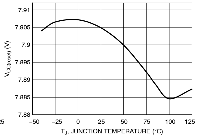
Figure 28. V CC(reset) vs. Temperature
