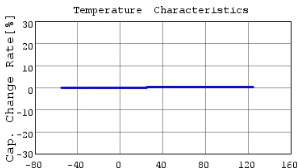
■ GJM1555C1H5R2CB01 C-Temp. capchange, DC0V, 1
