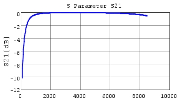
■ GJM1555C1H5R2CB01 S21 DC0V, 25degC
