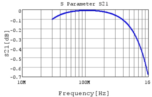
RHE5G2A331J0M1H03A S21 DCOV, 25degC
