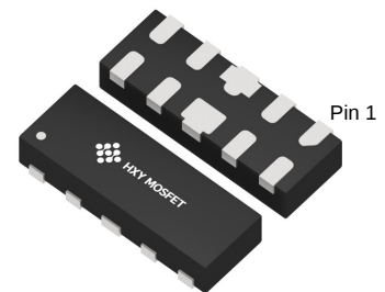
DFN2510-10L (DFN2510D-10))
