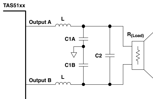
Figure 12. Demodulation Filter
