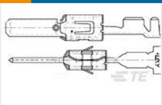
TE Part #185028-1 TAB F 2.8x0.8 CONTACT CS SWS Sn
