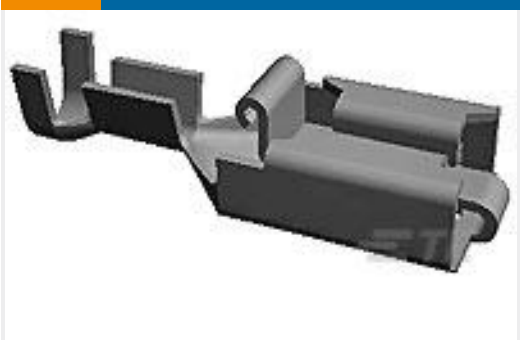
TE Part #927854-1 PL 250 REC TERMINAL 17-13 AWG BR
